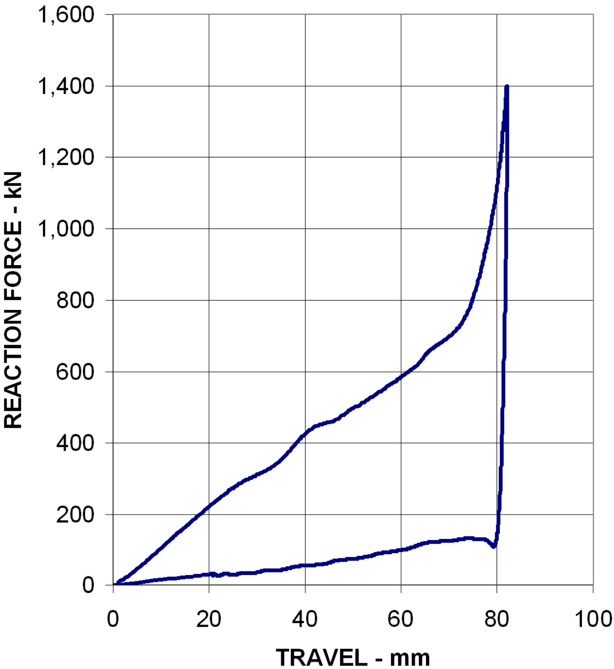
TF-880Q Dynamic Performance Curve
