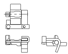
LOCK CATCH ASSEMBLY MKE10098
