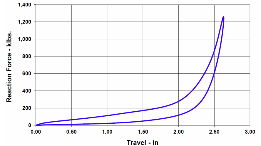
TP-17 Drop Hammer Performance
