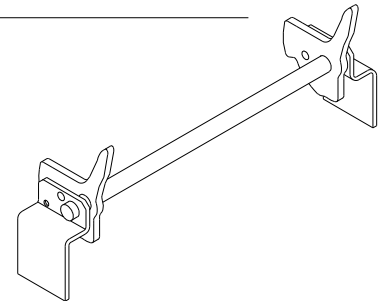
OPERATING SHAFT - 1 1/4 SQ. MKE7123
